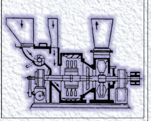
CROSS-SECTION OF IMPACT PULVERISER WITH WHIZER CONE CLASSIFIER.
