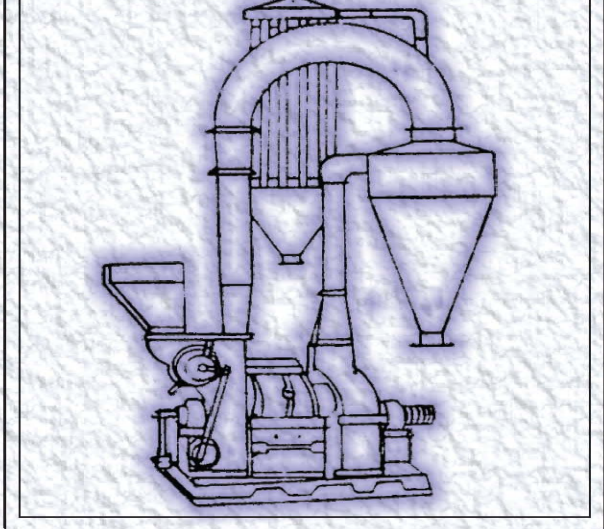
COMPLETE INSTALLATION WITH MILL, ROTARY FEEDER, CYCLONE COLLECTOR AND DUST COLLECTOR.
